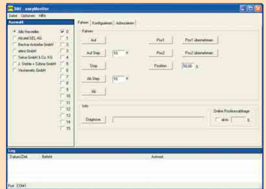
9 Diagnosetool SMI-easyMonitor
